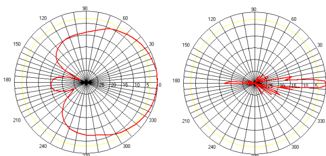
E Plane
