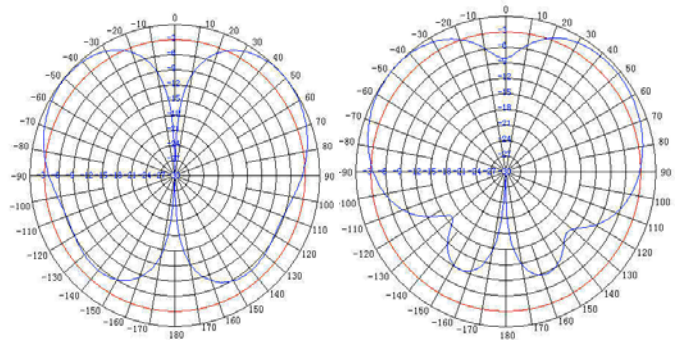
2.4GHz-E Plane
