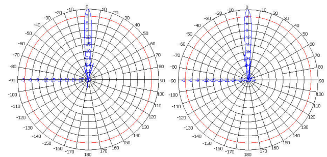
E Plane
